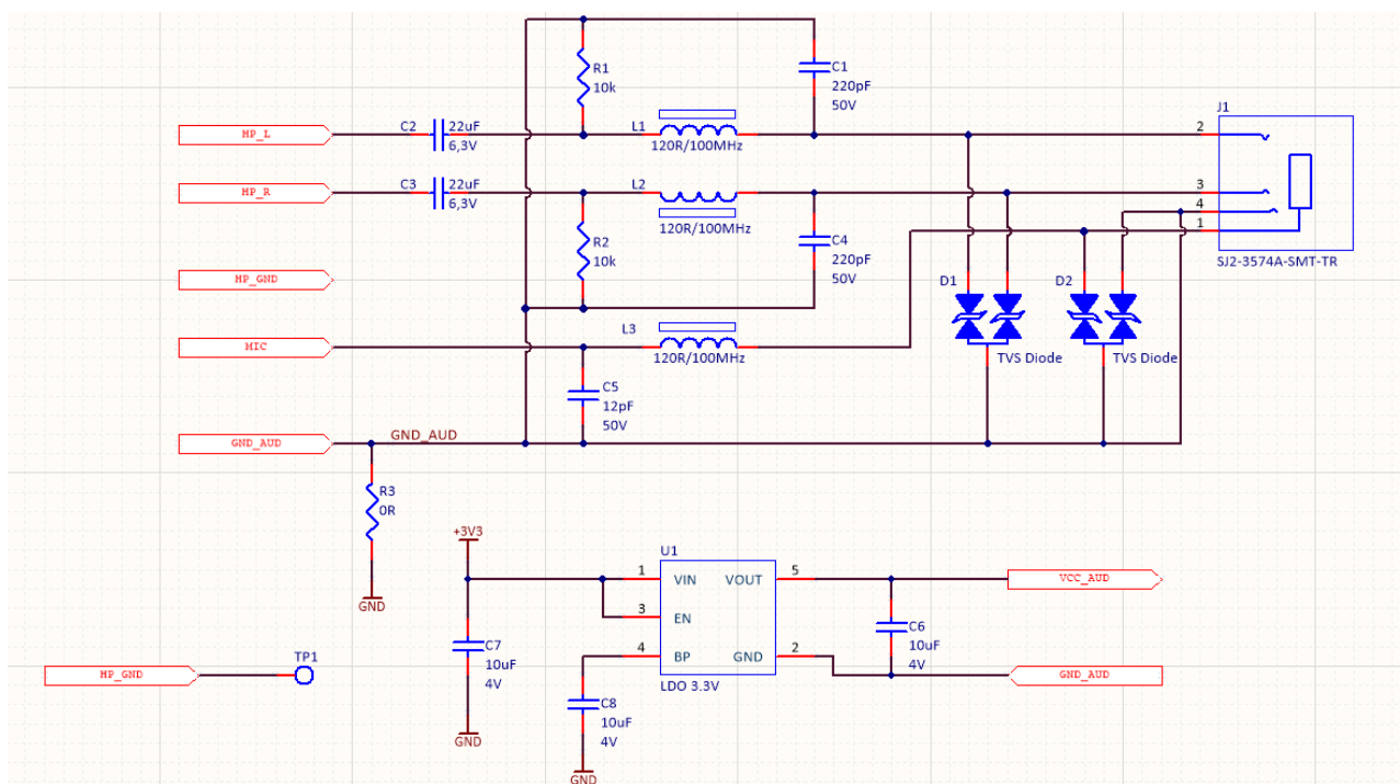
Figure 10: Headphone-Out Mic-In Example Circuit
