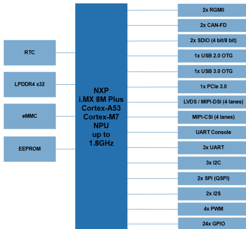
Figure 1: Block Diagram
