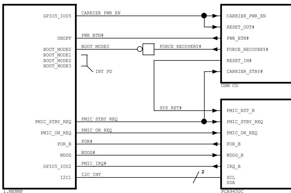
Figure 2: System Control (topology)
