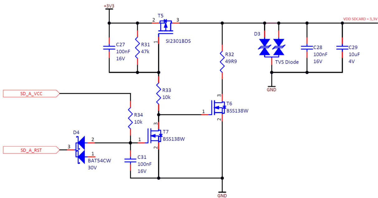
Figure 9: SD_A supply voltage switching circuit
