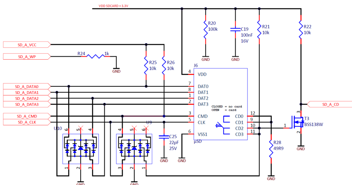
Figure 8: SD Card connector example connection
