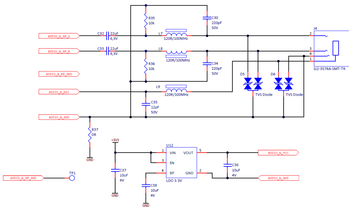
Figure 12: Headphone-Out Mic-In Example Circuit
