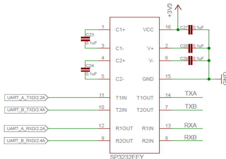
Figure 10: UART transceiver example
