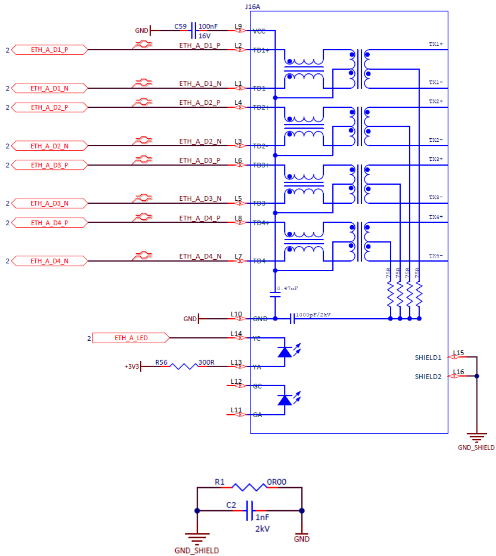
Figure 11: LAN output example
