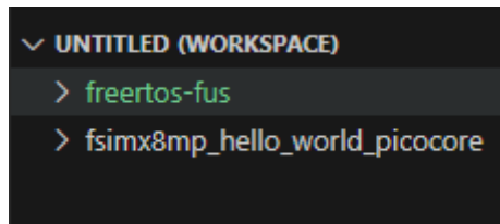
Figure 8: Imported examples
